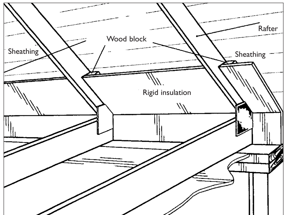
Figure 3 Insulating the outside edge of the attic floor
